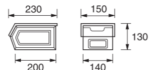
DIMENSIONI DIMENSION 230x140x130 h. CAPACITA' CAPACITY LT. 3,75
