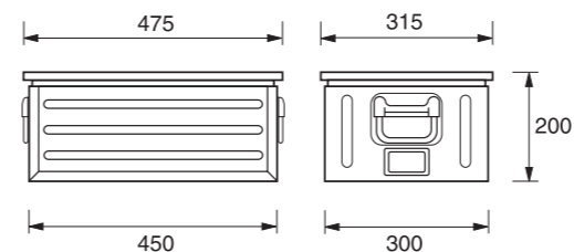
DIMENSIONI DIMENSION 450x300x200 h. CAPACITA' CAPACITY LT. 27
