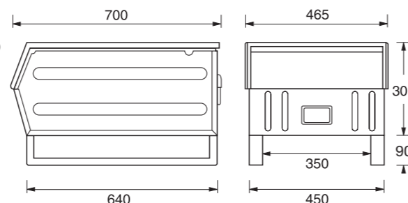
DIMENSIONI DIMENSION 700x450x390 h. CAPACITA' CAPACITY LT. 88
