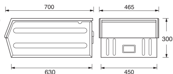
DIMENSIONI DIMENSION 700x450x300 h. CAPACITA' CAPACITY LT. 88
