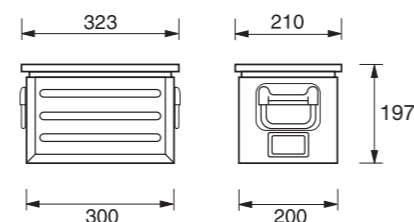
DIMENSIONI DIMENSION 300x200x197 h. CAPACITA' CAPACITY LT. 10
