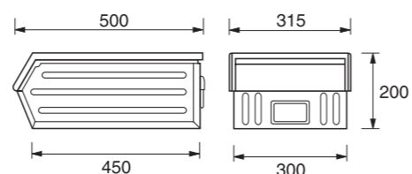
DIMENSIONI DIMENSION 500x300x200 h. CAPACITA' CAPACITY LT. 28
